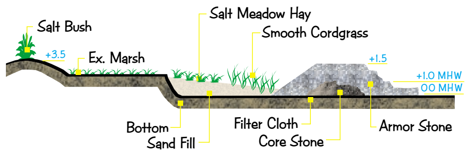
BREAKWATER SECTION A-A'
