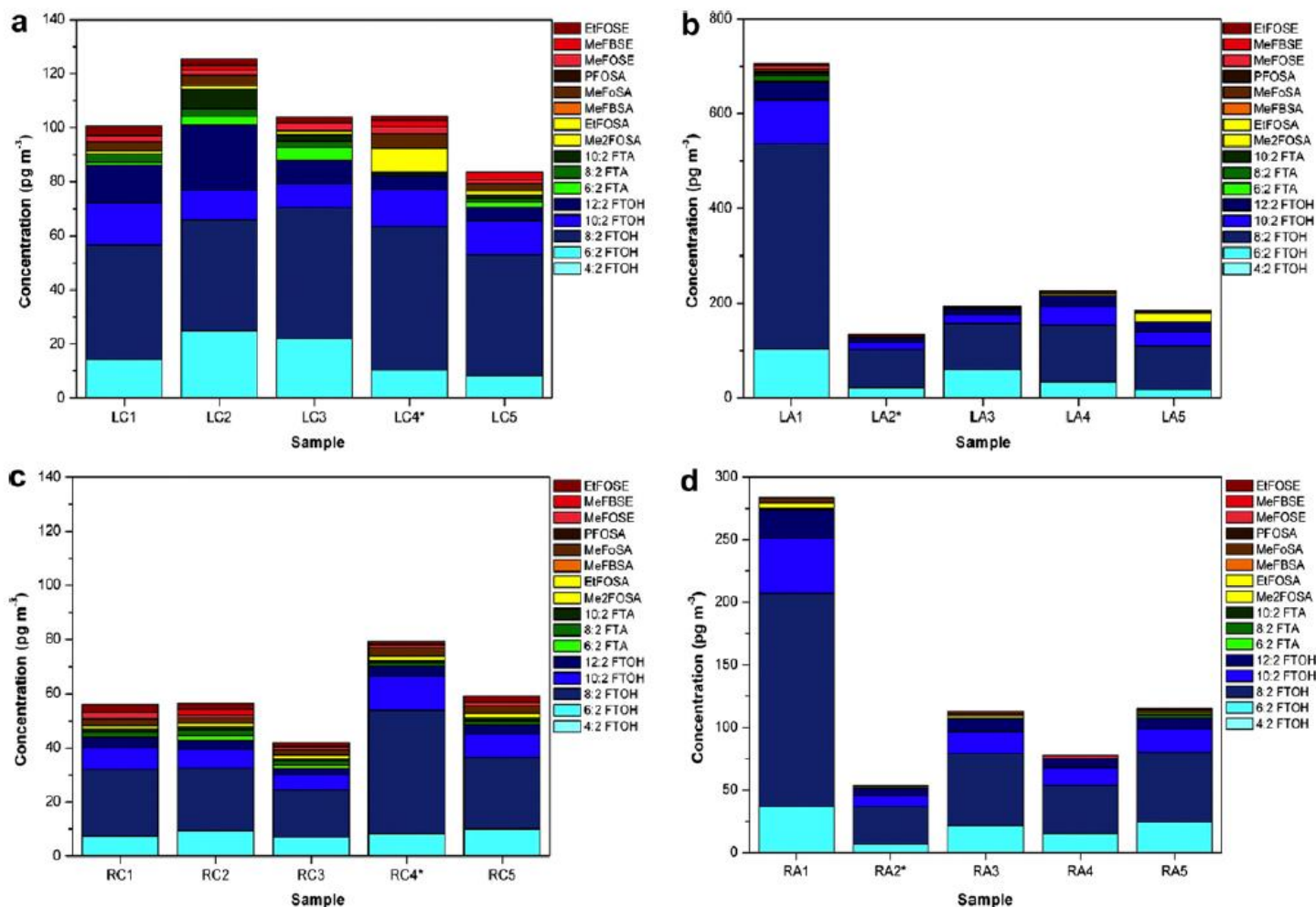
Fig. 1. Concentrations (pg m -3 ) of semi-volatile and volatile PFACs in gas-phase samples taken at landfills (LC (a) and LA (b)) and at the corresponding reference sites (RC(c) and RA (d)). Sampling periods: 11.08.–18.08.2009 (LC) and 27.08.–02.09.2009 (LA). Note the different scales. Asterisks mark the 3-day samples.
