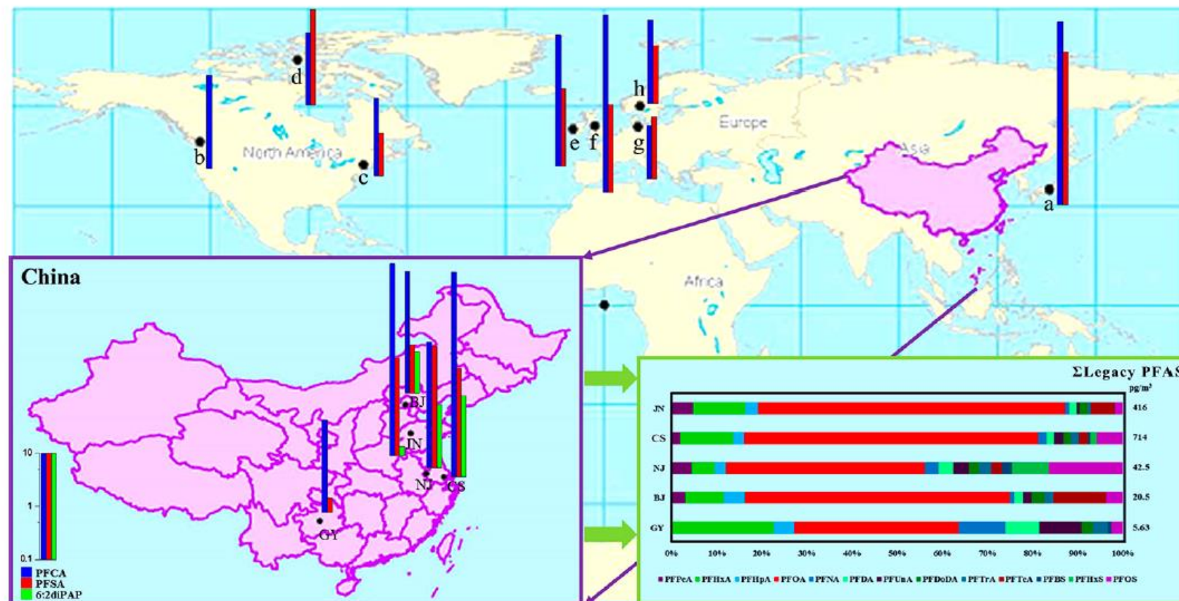
Figure 3. Distribution of PFCAs, PFSA, and 6:2 diPAP in outdoor APM (data for China were obtained from this study, and those for other countries were obtained from previous studies; a: Japan, 76 b: Canada, 29 c: U.S., 77 d: Arctic, 78 e: UK, 42 f: Ireland, 42 g: Germany, 79 h: Norway 42 ) and proportional distribution of legacy PFASs in outdoor APM (value of legacy PFASs is arithmetic mean).
