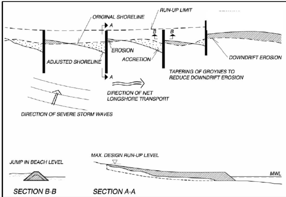
Figure 5-7: Typical configuration of a series of groins. (Burcharth and Hughes 2002)
